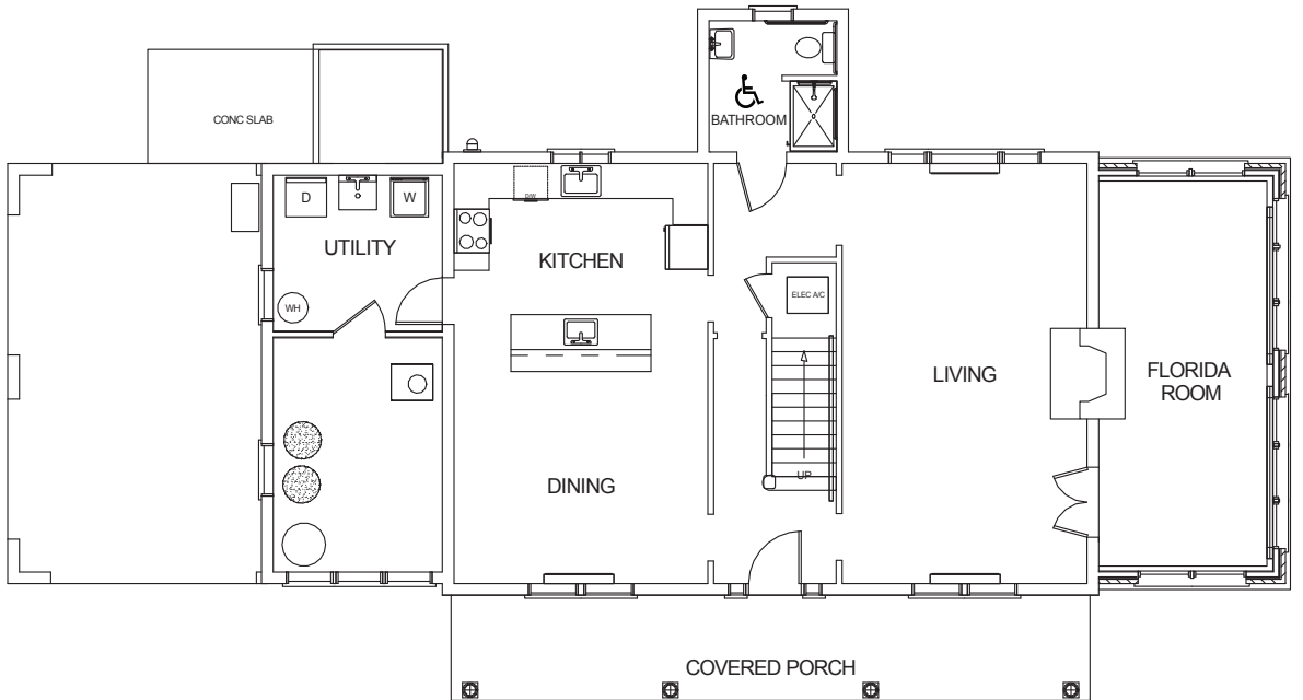
FIRST FLOOR
